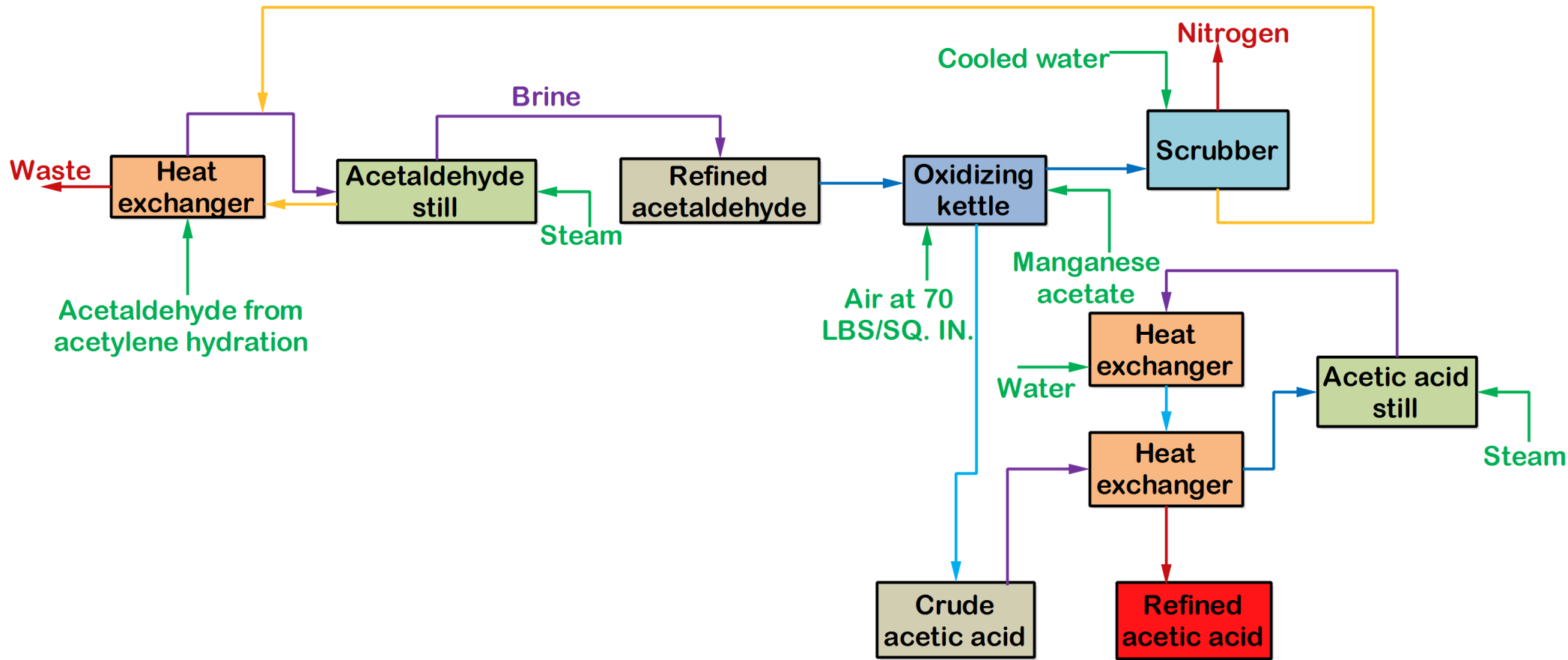
Figure: Manufacture of acetic acid from acetaldehyde
